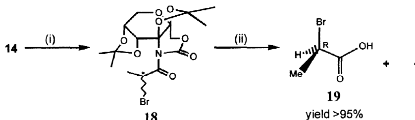
Scheme 5. Reagents and conditions: (i), THF, NBS, -78°C; (ii), LiOH, H 2 O 2 , 0°C.
