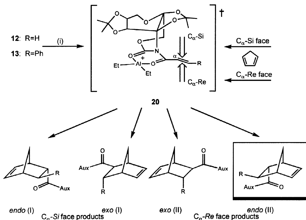
Scheme 6. Reagents and conditions: (i), \text{CH}_2\text{Cl}_2 , cyclopentadiene (10 eq), \text{Et}_2\text{AlCl} (1.4 eq) 12 : -78^{\circ}\text{C} , 13 : -20^{\circ}\text{C}
