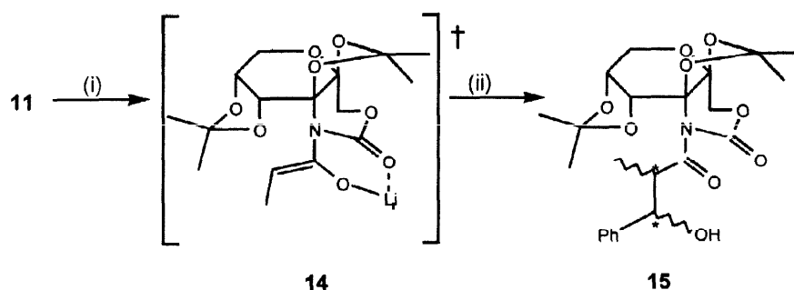
Scheme 3. Reagents and conditions: (i), \text{LiNPr}_2 , THF, 0^\circ\text{C} ; (ii), \text{PhCHO} , THF, 0^\circ\text{C} .
