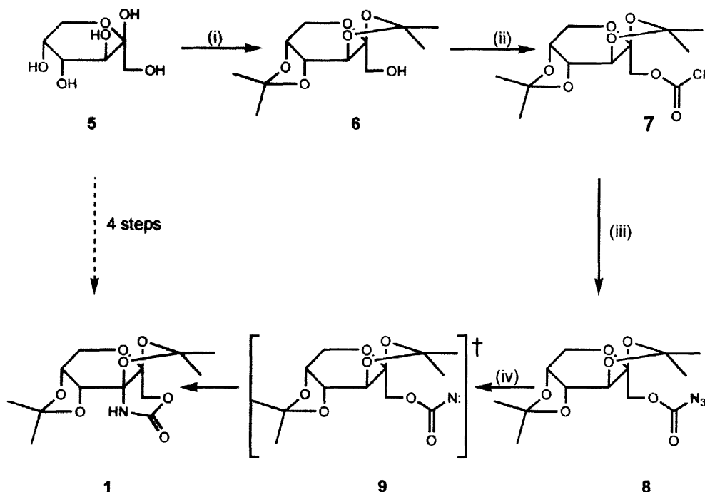
Scheme 1. Reagents and conditions: (i), acetone/conc. \text{H}_2\text{SO}_4 ; (ii), \text{Cl}_2\text{CO} /pyridine; (iii), \text{NaN}_3 /TBAB; (iv), TCE/reflux 147^\circ\text{C} .
