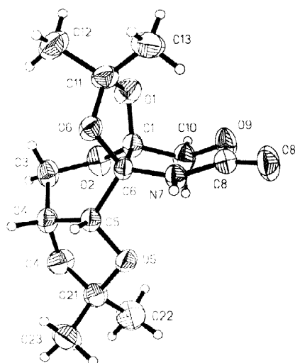
Figure 1. (a) View of the X-ray crystal structure of 1,3-oxazin-2-one 1 and (b) of aldol-adduct 15 . The molecules of 1 and 15 are shown as 40% thermal ellipsoid plots.
