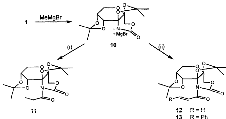
Scheme 2. Reagents and conditions: (i), \text{MeMgBr} , \text{Et}_2\text{O} , 0^\circ\text{C} ; (ii), THF, -78^\circ\text{C} , \text{EtCOCl} ; (iii), THF, -78^\circ\text{C} , \text{RCH=CHCOCl} .
